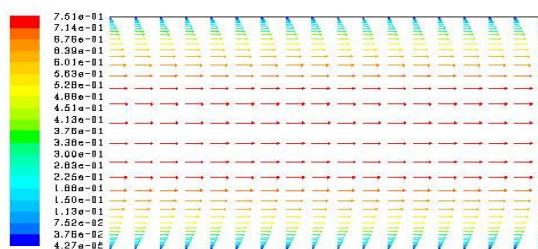
Fig. 5 Distribution of velocity vectors at the output
