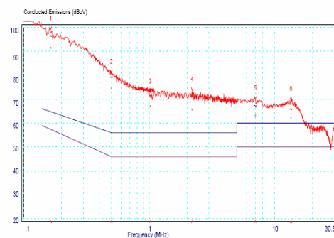
Fig.6 Conducted Emissions without Common Mode Filter
