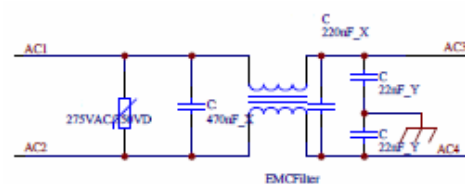
Fig. 5 Inbuilt EMC filter (1 phase 240V, 2.2KW VSD)
