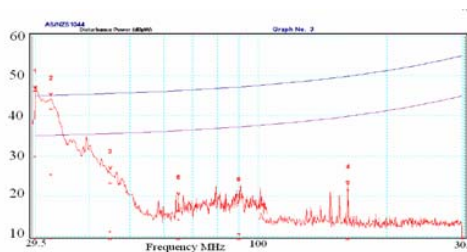
Fig.9 Disturbance Power (System with Filter)
