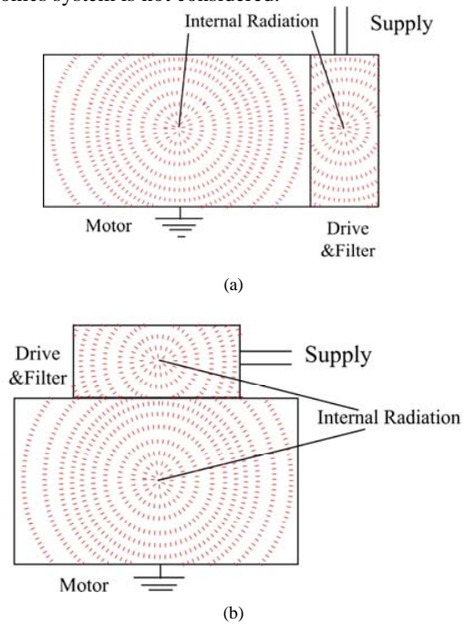
Fig.3 Position of Drive with respect to Motor
