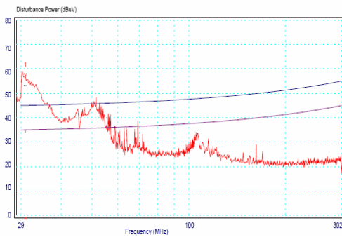
Fig.8 Disturbance Power (System without Filter)
