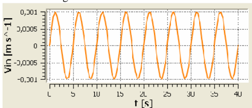
Fig.9 Inlet velocity
