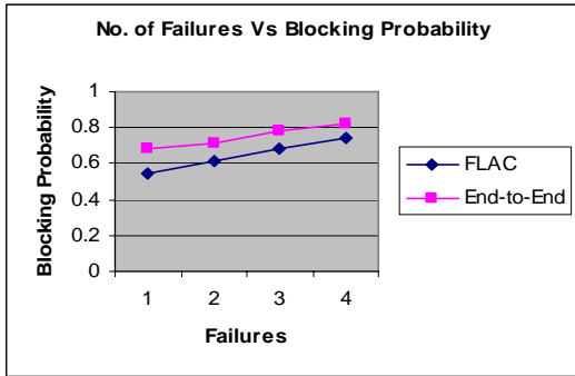
Fig. 3 No. of Failures Vs Blocking Probability
