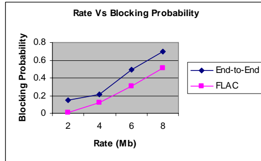
Fig. 6 Rate Vs Blocking Probability
