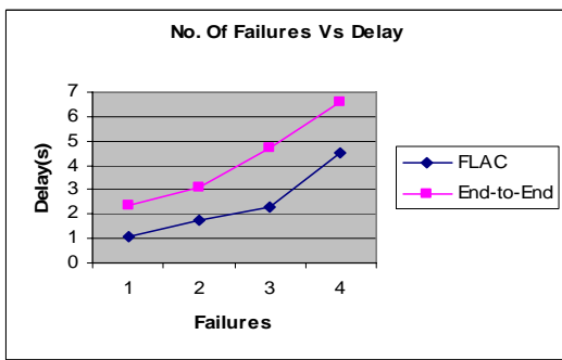
Fig. 4 No. of Failures Vs Delay
