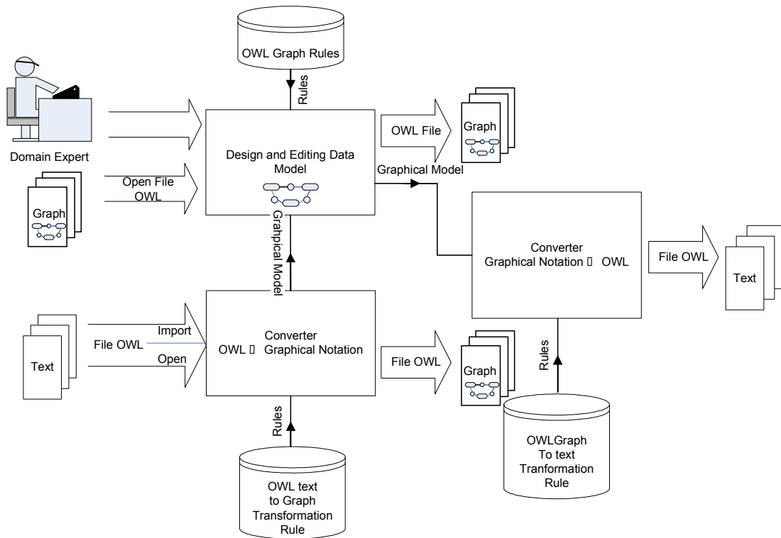
Fig. 5 System Architecture
