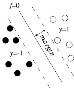
Fig. 1. Linear separation of the labeled training data by using the hyperplane f = 0 .
