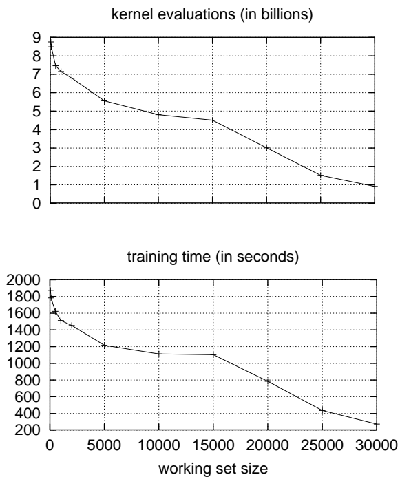
Fig. 4. Number of kernel evaluations and training time for different values of \hat{l} .
