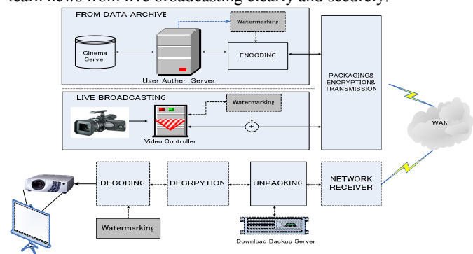
Fig 1 Digital Cinema system
