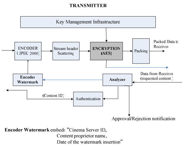
Fig 2 Transmitter LSI with encryption method JPEG2000 compatible transmitter is responsible for inputs from both the digitalized data from the Cinema server and watermarking data at the same time. The plain content and Watermark data are added inside the Encoder by our Crc-32
