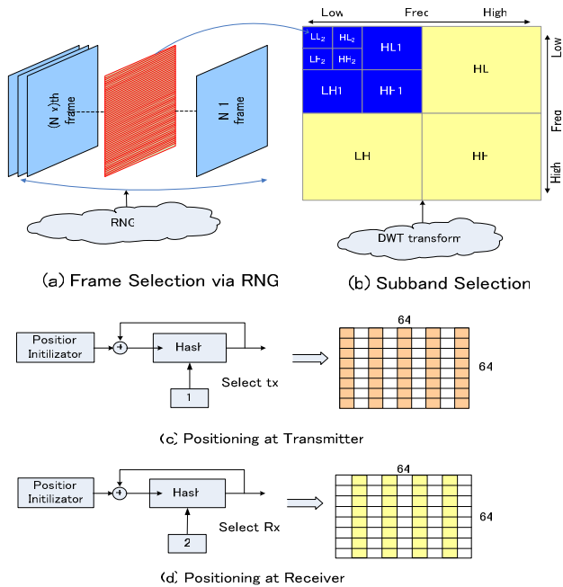
Fig 6 Watermarking Algorithm
