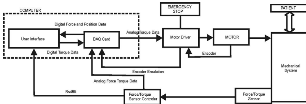
Fig. 5 System Hardware Block Scheme
