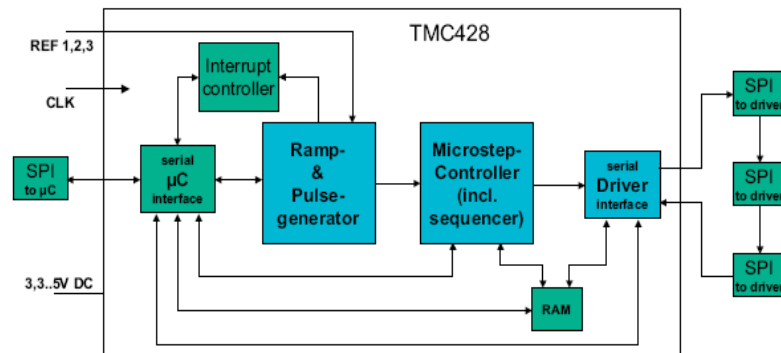
Fig. 7 Three Axis Stepper Motor Controller Block Scheme
