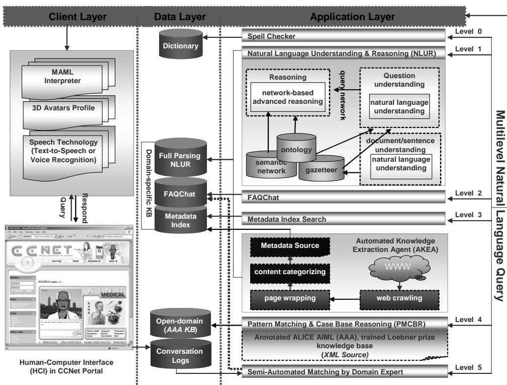
Fig. 1 AINI's Conversational Agent Architecture
