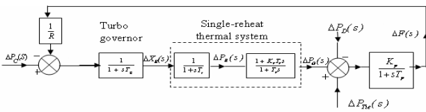
Fig. 1 Transfer Function Model of Singe-Reheat Thermal System
