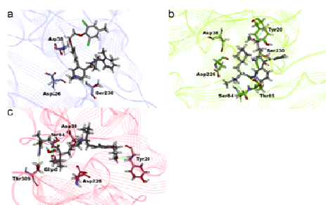
Fig. 4 Binding mode of each inhibitor in three representative structures.
