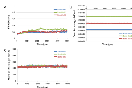
Fig. 2 Results of simulation stability analyses for three systems. a Ca RMSD with respect to the initial structure, b the potential energy, and c the number of intra-protein hydrogen bonds are plotted throughout the 5 ns MD simulation
