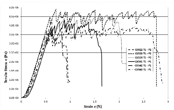
Fig. 6 Stress-strain results for specimens tested in tension: effect of process type (Fiber type 1)
