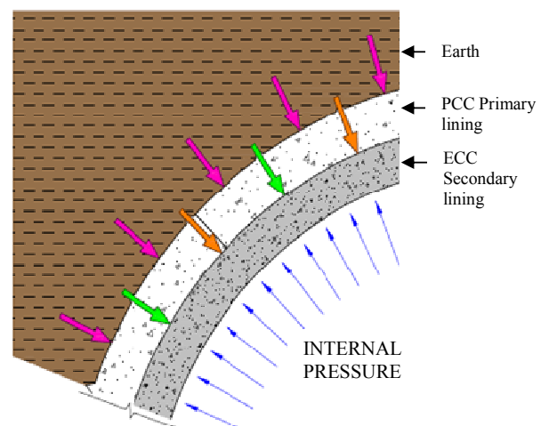
Fig. 1 ECC tunnel lining for repair
