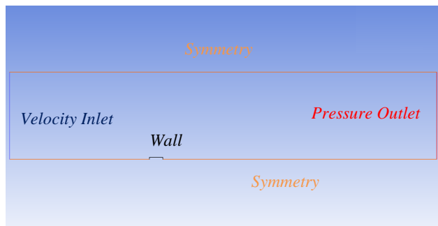
Fig. 8 Boundary conditions of the computational domain
