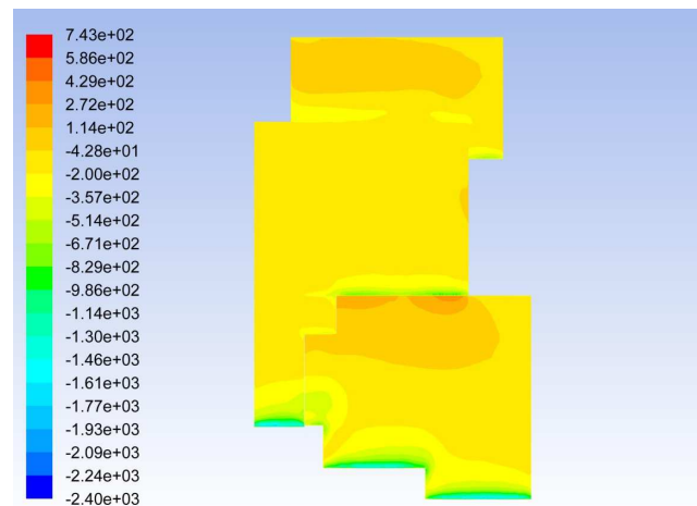
Fig. 6 Static pressure distribution [Pa] on top of the SMART centre for an incoming South wind
