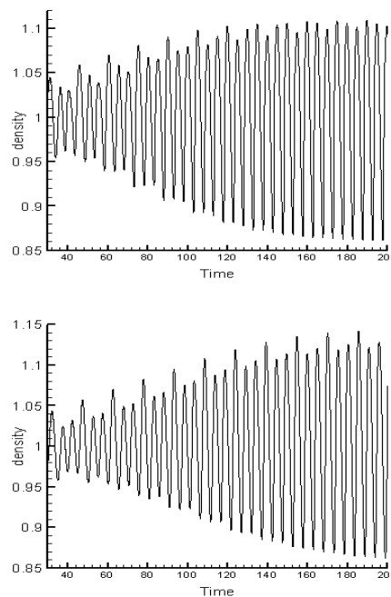
Fig. 9 Density fluctuations at (x,y) = (8,1.5)D for the open cavity without the rear wall treatment (9a) and with the rear wall treatment (9b). The rest of the conditions are as in Fig. 4
