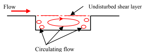
Fig. 1 Illustration of an open-cavity
