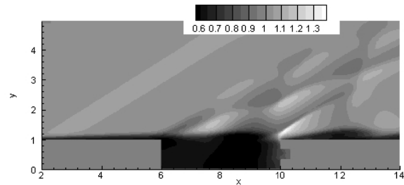
Fig. 5 Instantaneous density fluctuation contours for an open cavity with a rear wall treatment of a square hole of a length of D/3 . The rest of the conditions are as in Fig. 4
