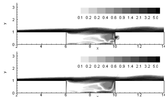
Fig. 6 Instantaneous vorticity magnitude contours for the open cavity without the rear wall treatment (6a - upper) and with the rear wall treatment (6b - lower). The rest of the conditions are as in Fig. 4
