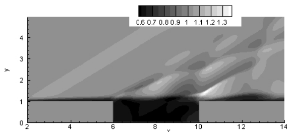
Fig. 4 Instantaneous density fluctuation contours for an open cavity of L/D=4 at time 175. The depth D has been normalised to one
