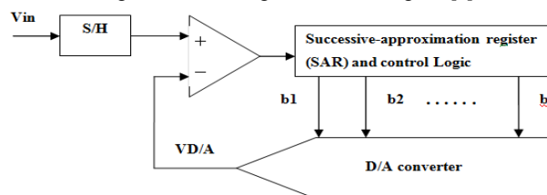
Fig. 2 SAR architecture
