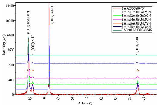
Fig. 1 XRD Phase analysis of \text{In}_x\text{Al}_y\text{Ga}_{1-x-y}\text{N} quaternary alloys
