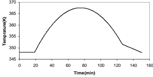
Fig. 2 Temperature Profile
