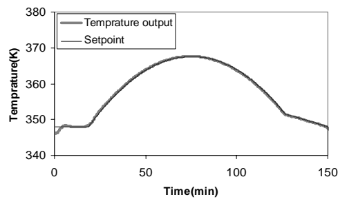
Fig. 7 The MPC controller Response
