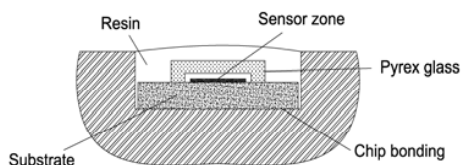
Fig. 7 Schematic view of sensing chip with packaging components
