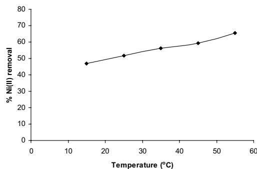
Fig. 8 Effect of temperature on Ni(II) removal [Ni(II) conc = 100 mg L -1 ; adsorbent dose = 20.0 g L -1 ; pH = 6.0; contact time = 180 min; stirring speed = 180 rpm]
