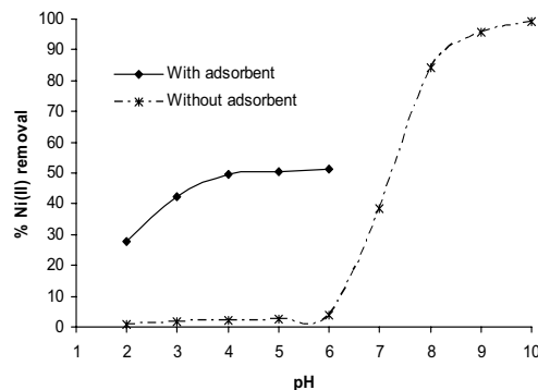
Fig. 4 Effect of pH on Ni(II) removal [Ni(II) conc = 100 \text{ mg L}^{-1} ; adsorbent dose = 20.0 \text{ g L}^{-1} ; contact time = 180 min; stirring speed = 180 rpm; temp = 25^\circ\text{C} ]
