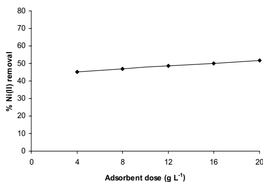
Fig. 5 Effect of adsorbent dose on Ni(II) removal [Ni(II) conc = 100 \text{ mg L}^{-1} ; pH = 6.0; contact time = 180 min; stirring speed = 180 rpm; temp = 25^\circ\text{C} ]
