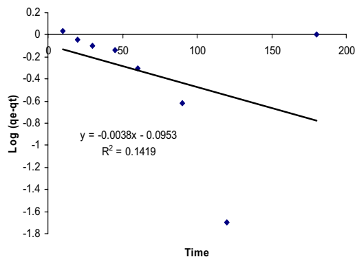
Fig. 12 Pseudo-first order model for Ni(II) adsorption [initial Ni(II) conc = 100 mg L -1 ; contact time = 10-180 min]
