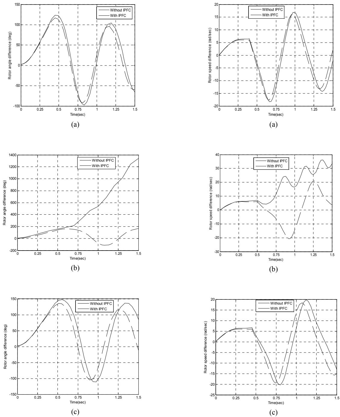
Fig. 4 Variation of generator – 2(6 bus system) rotor angle difference without and with IPFC for different fault clearing times( t_c ), (a) t_c = 0.4 (b) t_c = 0.5 (c) t_c = 0.45
