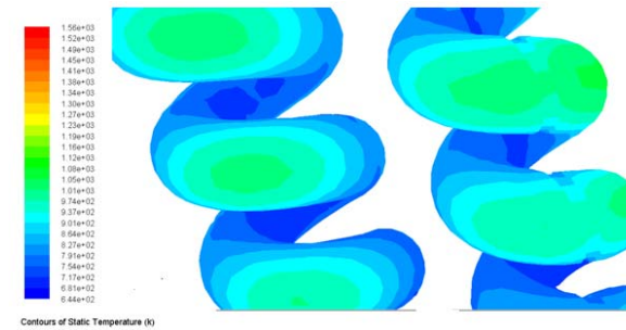
Fig. 9 Contours of static temperature for cooling ducts having turbulators of e/D = 0.04 and 0.75mm rib thickness
