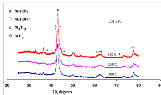
Fig. 4 XRD patterns of the SHS-synthesized porous NiTi SMAs at a chamber pressure of 201 kPa with different preheating temperatures of 200°C, 250 °C and 300°C
