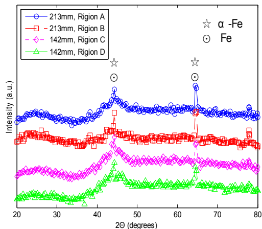
Fig. 5 XRD measured results of different ribbon samples
