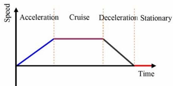
Fig. 1 Ideal speed profile for stop/start cycle
