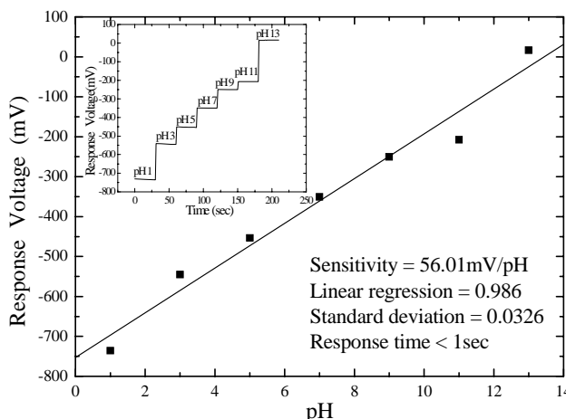
Fig. 2 Sensitivity of RuO 2 array sensors at 25°C
