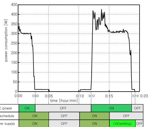
Fig. 9. Measured power consumption of a outlet connected a PC on schedule
