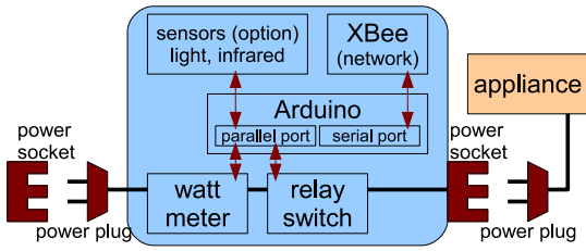
Fig. 2. Configuration of the multifunctional electrical outlet
