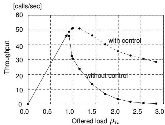
Fig. 7 Throughput characteristics
