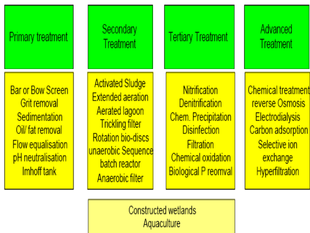
Fig. 2 Wastewater treatment categories and technologies
