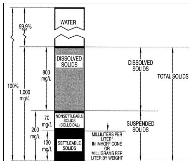
Fig. 1 Composition of solids in wastewater
