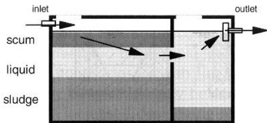
Fig. 4 Septic Tank
