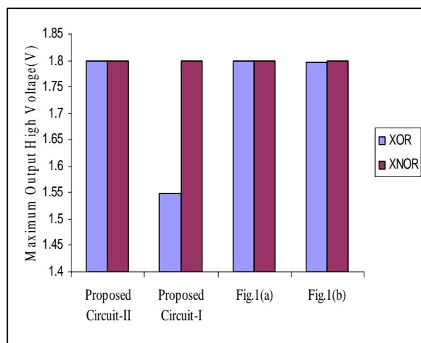
Fig. 7(b) V_{OH} of different XOR-XNOR circuits at 1.8V supply voltage
