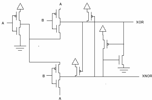
Fig. 4 Proposed XOR-XNOR circuit-II
