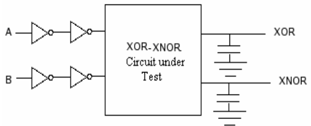
Fig. 5 Simulation test bench
