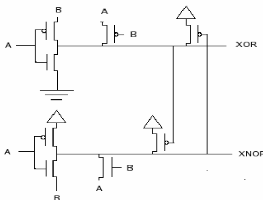
Fig. 2 Proposed XOR-XNOR circuit-I
