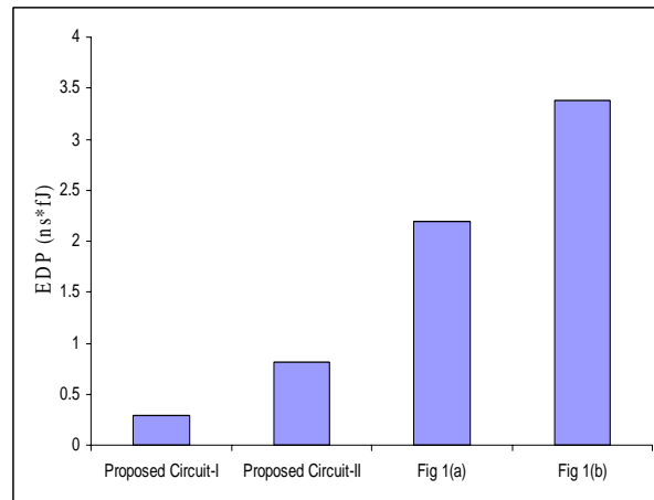
Fig. 6(f) EDP of different XOR-XNOR circuits at 1.8V supply voltage
