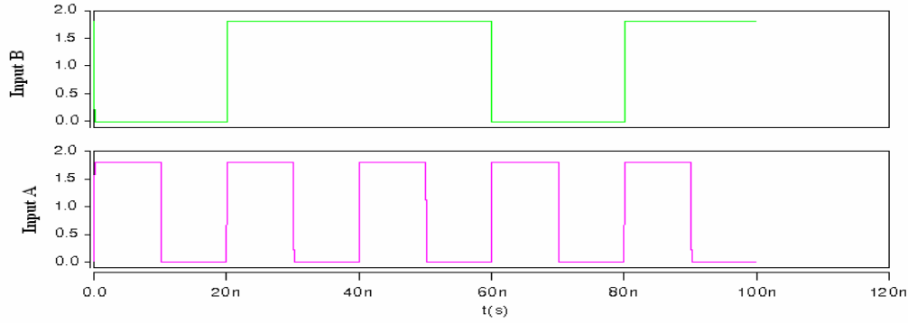
Fig. 3(a) Input waveforms for the proposed circuits
