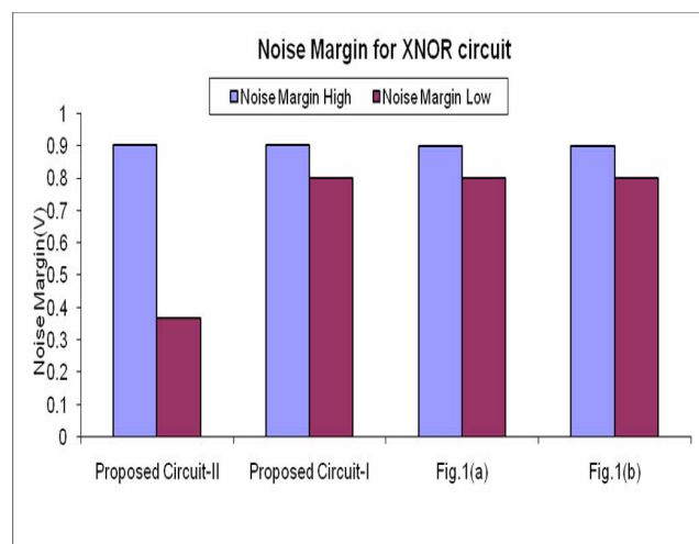
Fig. 7(d) Noise Margin of different XNOR circuits at 1.8V supply voltage
