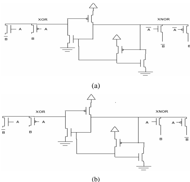
Fig. 1 XOR-XNOR circuits reported in [16]
