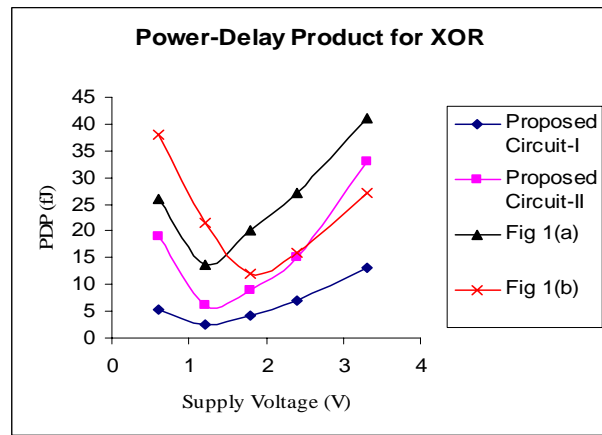
Fig. 6(d) PDP Vs supply voltage graph for different XOR circuits
