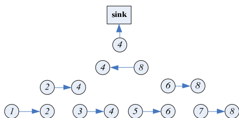
Fig. 3 Chain in PEGASIS
