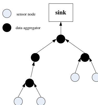
Fig. 4 Tree-based structure
