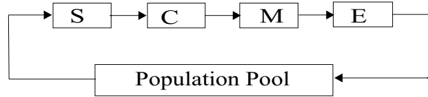
Fig. 1. Pipeline stages for the GA. Here S, C, M and E stand for selection, crossover, mutation and evaluation respectively
