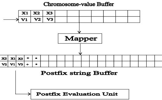
Fig. 4. Postfix evaluation scheme for GA fitness function
