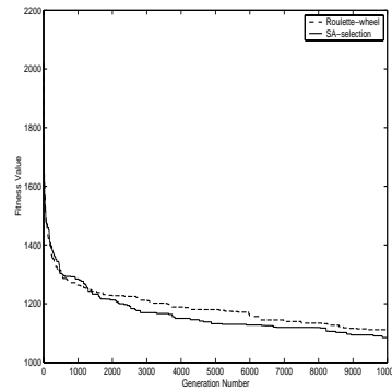
Fig. 17. Convergence of f_F using roulette-wheel and SA-selection when problem dimension = 125
