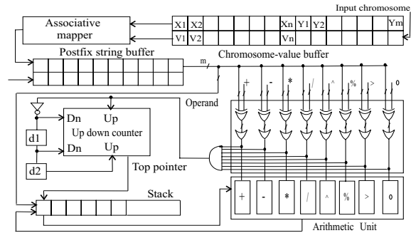
Fig. 5. Evaluation unit for general optimization
