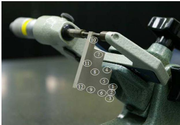
Fig. 6 Measurement position
