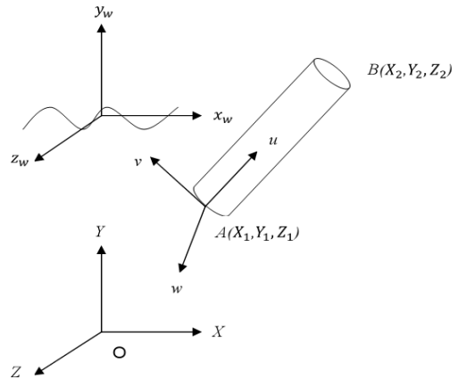
Fig. 2 Reference systems
