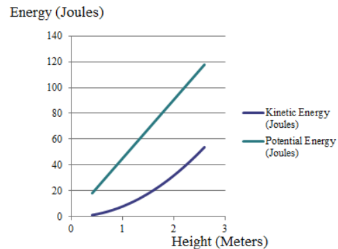
Fig. 2 Kinetic and Potential Energies with 65kg Mass
