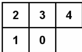
Fig. 3. Pixel position
