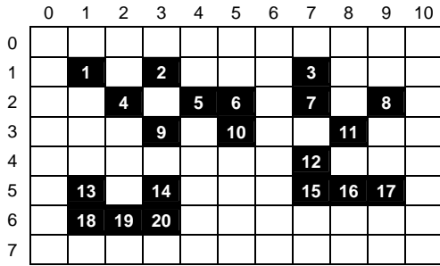
Fig. 7 Pixels Position
