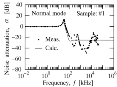
Fig. 7 Normal mode noise attenuation characteristics.
