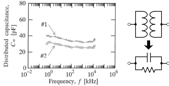
Fig. 5 Frequency characteristics of distributed capacitance between the primary and secondary windings.
