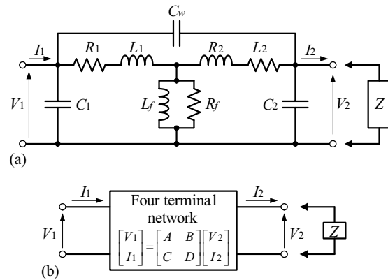
Fig. 6 Equivalent circuit of the transformer. (a) Normal mode equivalent circuit. (b) Four terminal network.
