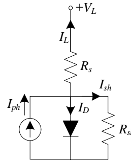
Fig. 2 Equivalent circuit of a single diode model
