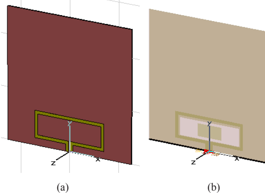
Fig. 2 Proposed microstrip loop antenna (a) top view (d) bottom view with defective ground plane
