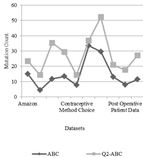
Fig. 3 ABC and Q 2 ABC execution energy efficiency
