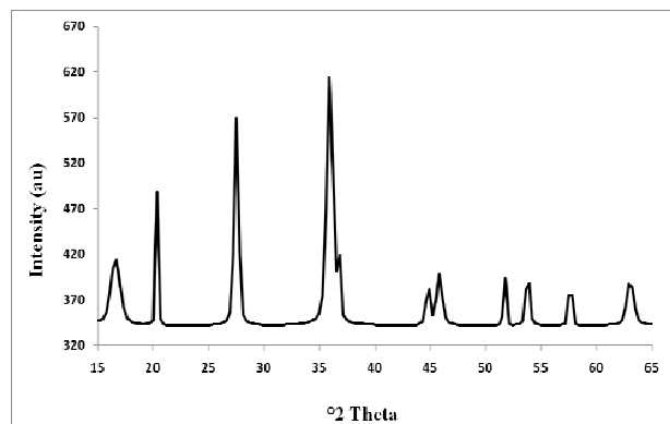
Fig. 5 XRD diffraction patterns of isolated magnetosomes
