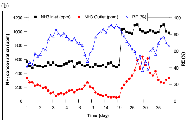
Fig. 3 Relationship between ammonia inlet, ammonia outlet and removal efficiency at manure fertilizer: bagasse ratio (a) 1:3 ratio (b) 1:5 ratio (c) 1:7 ratio
