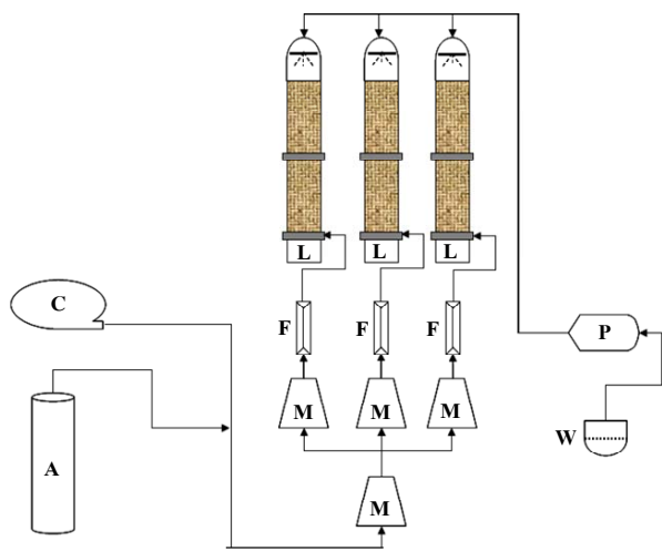
Fig. 2 Flow diagram of biofiltration process (A= NH 3 gas tank, C= compressed air equipment, F = flow meter, L = Leachate tank, M = mixed air and NH 3 gas tank, P = peristaltic pump, and W = water tank)
