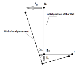
Fig. 4 Displacement Pattern of the Wall
