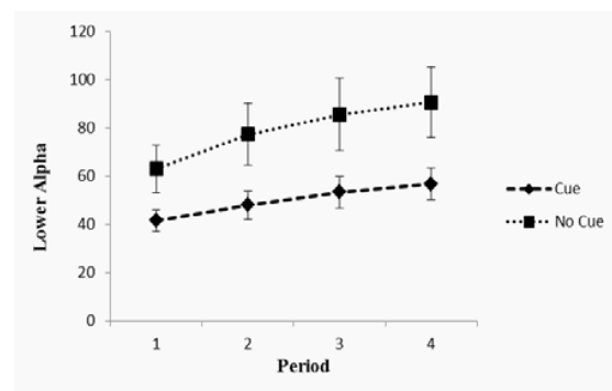
Fig. 4 Lower frequency alpha index of vigilance task
