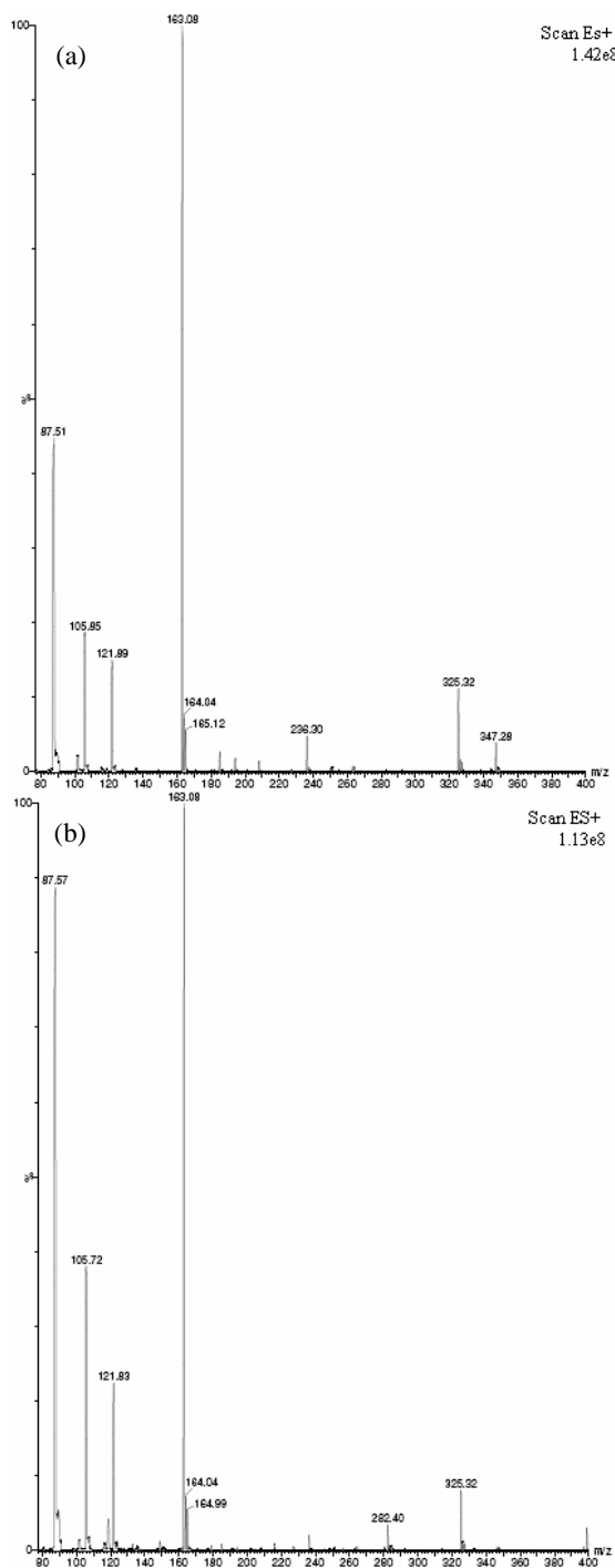
Fig. 4 Mass spectrometry of methomyl degradation of at the reaction time of (a) 0 minute, and (b) 30 minutes, by Fenton reagents H_2O_2 and Fe^{2+} of 1.0 mM and 0.5 mM, respectively
