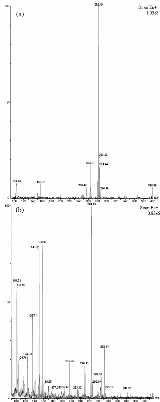
Fig. 5 Mass spectrometry of parathion degradation of at the reaction time of (a) 0 minute, and (b) 30 minutes, by Fenton reagents H_2O_2 and Fe^{2+} of 1.0 mM and 0.5 mM, respectively
