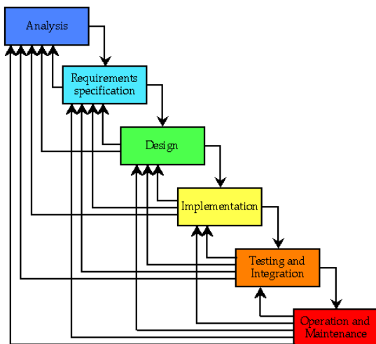
Fig. 1 Software lifecycle
