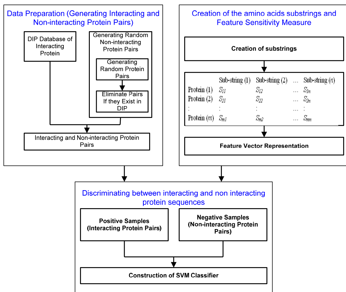
Fig. 1 algorithm overview
