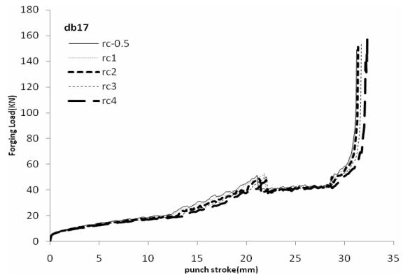
Fig.15. Effect of die corner radius on forging load
