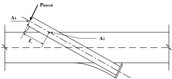
Fig. 8 Lateral load to the axis of the fixing pipe
