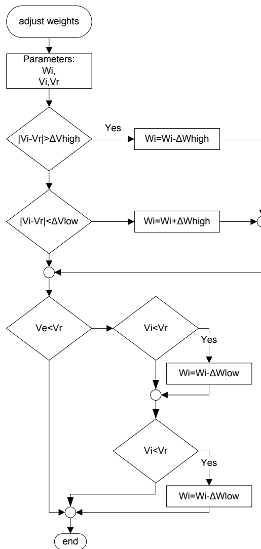
Fig. 4. DFD for weight adjustment
