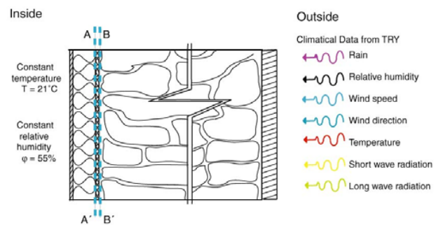
Fig. 2 Boundary conditions for the studied envelopes
