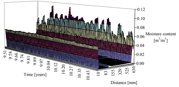
Fig. 6 Moisture content in sandstone wall, MW-hard
