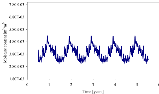
Fig. 15 Moisture content in the B-B' profile, sandstone wall, MW-soft
