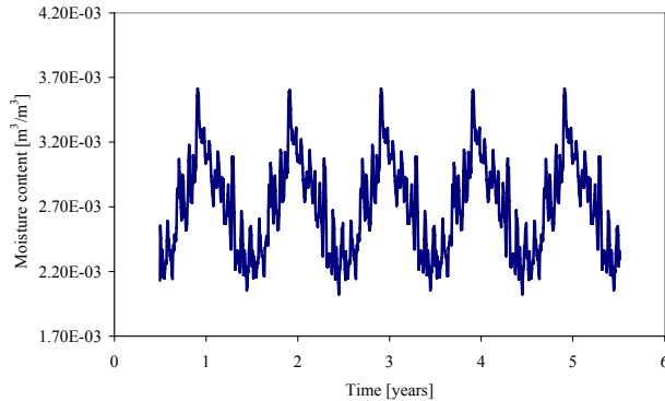
Fig. 14 Moisture content in the A-A' profile, sandstone wall, MW-soft
