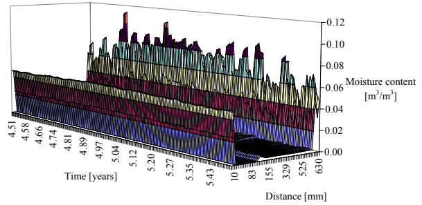
Fig. 13 Moisture content in sandstone wall, MW-soft
