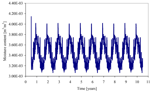
Fig. 8 Moisture content in the B-B' profile, sandstone wall, MW-hard
